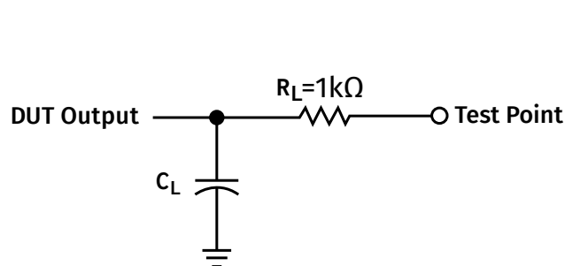
Figure 3: Load Circuit
