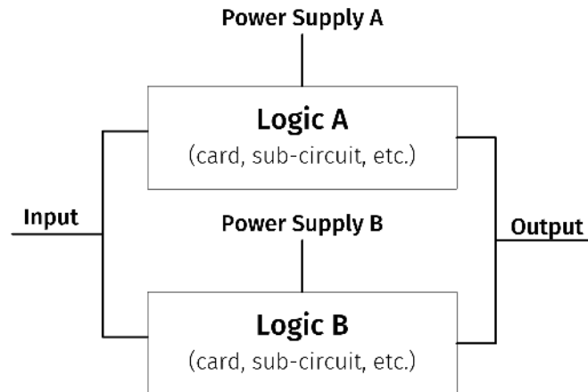
Figure 9: Two-Path Cold-Sparing Configuration
