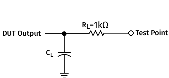
Figure 5: Load Circuit
