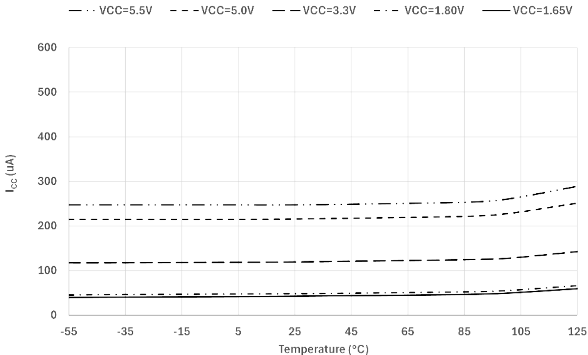
Figure 3: AP54RHC08 Typical I_{CC} vs. Temperature at 0krad TID (1)
