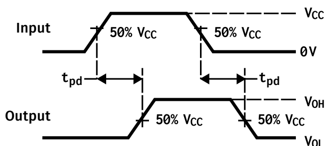
Figure 6: Propagation Delay Measurement
