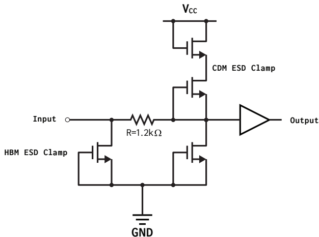
Figure 7: Input Pin Structure
