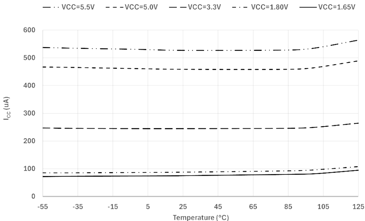
Figure 4: AP54RHC08 Typical I_{CC} vs. Temperature at 30krad TID (1)
