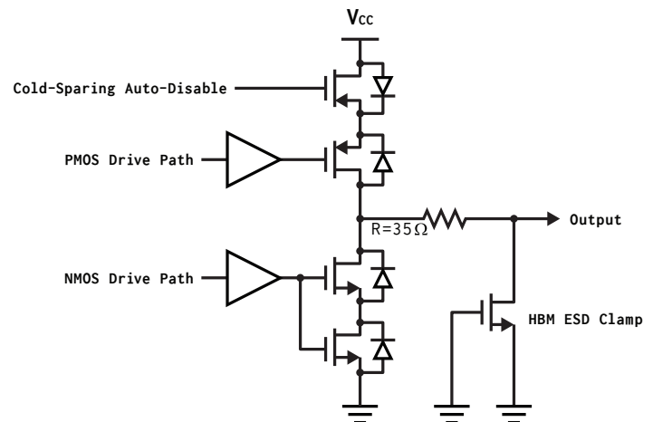
Figure 8: Output Pin Structure
