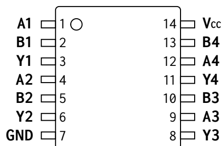
Figure 2: AP54RHC08 Device Pinout
