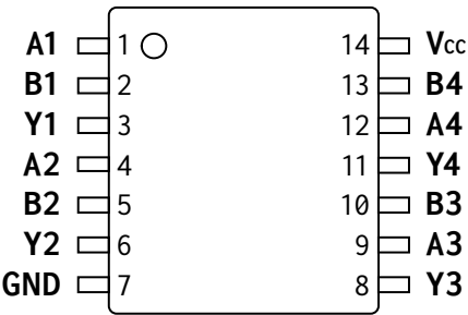
Figure 2: AP54RHC08 Device Pinout
