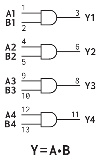
Figure 1: AP54RHC08 Logic Diagram
