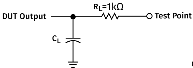
Figure 4: Load Circuit
