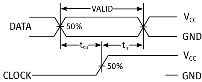
Figure 7: Setup And Hold Time
