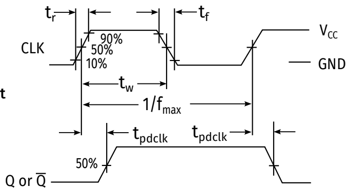
Figure 5: Clock Setup
